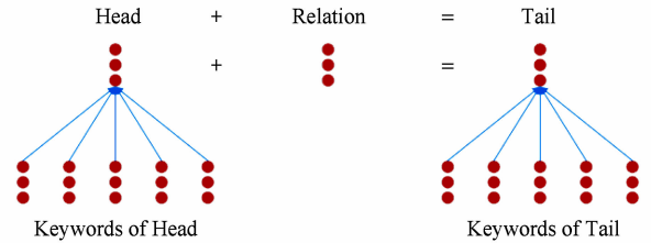
Fig. 10 DKRL (CBOW) model.
