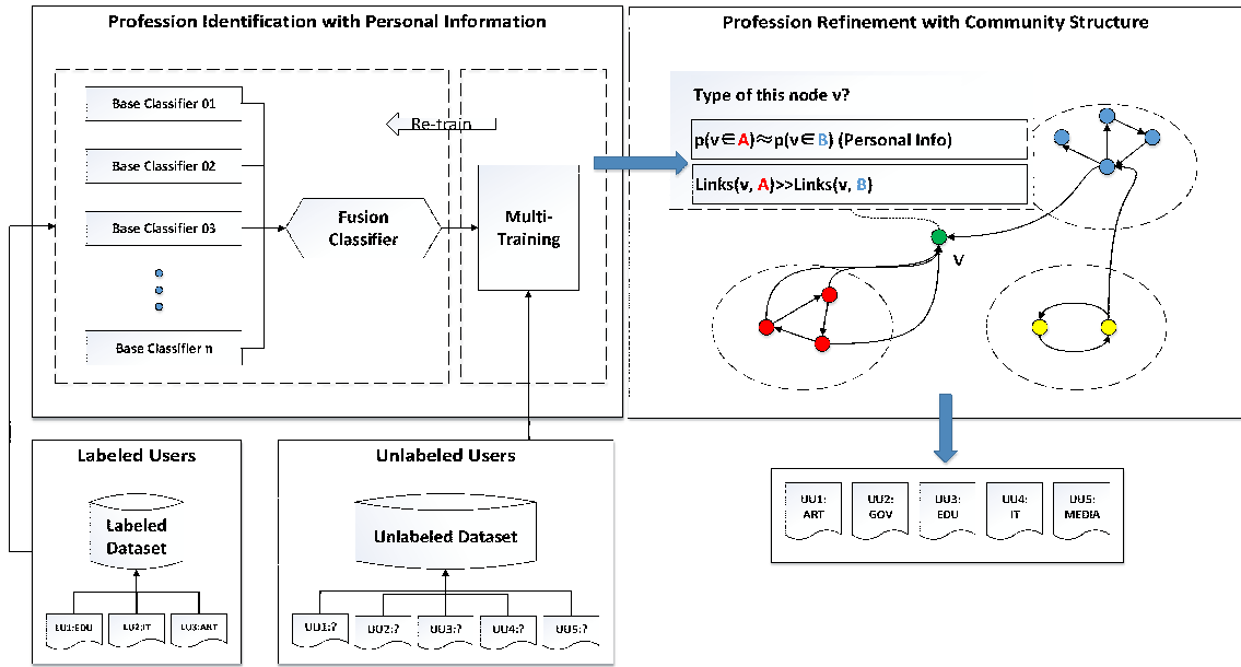
图 2.1 The framework of PRISM.
