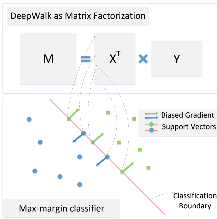
图 4.2 An illustration of Max-Margin DeepWalk.
